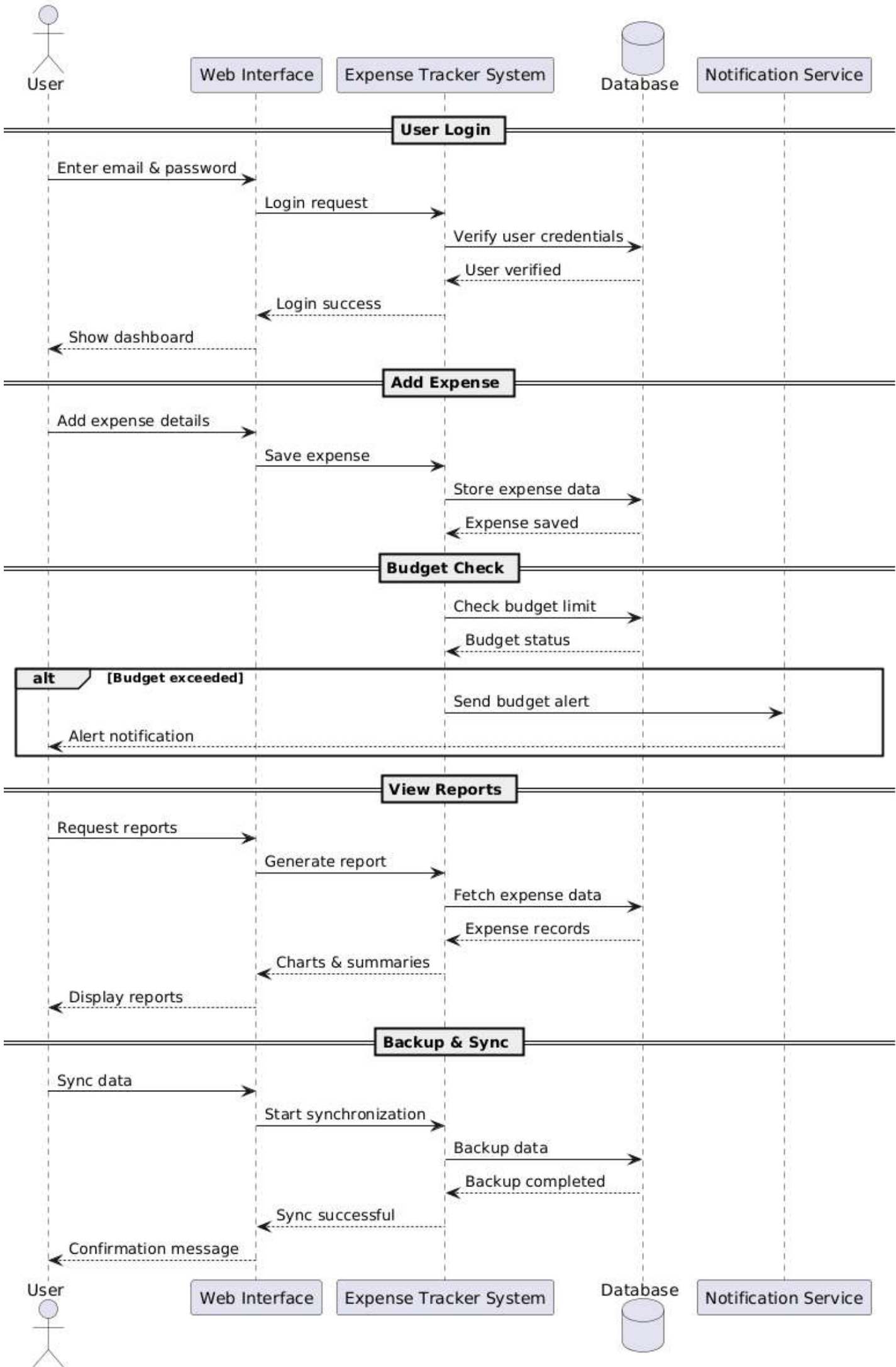
Sequence Diagram For Expense Tracker System
