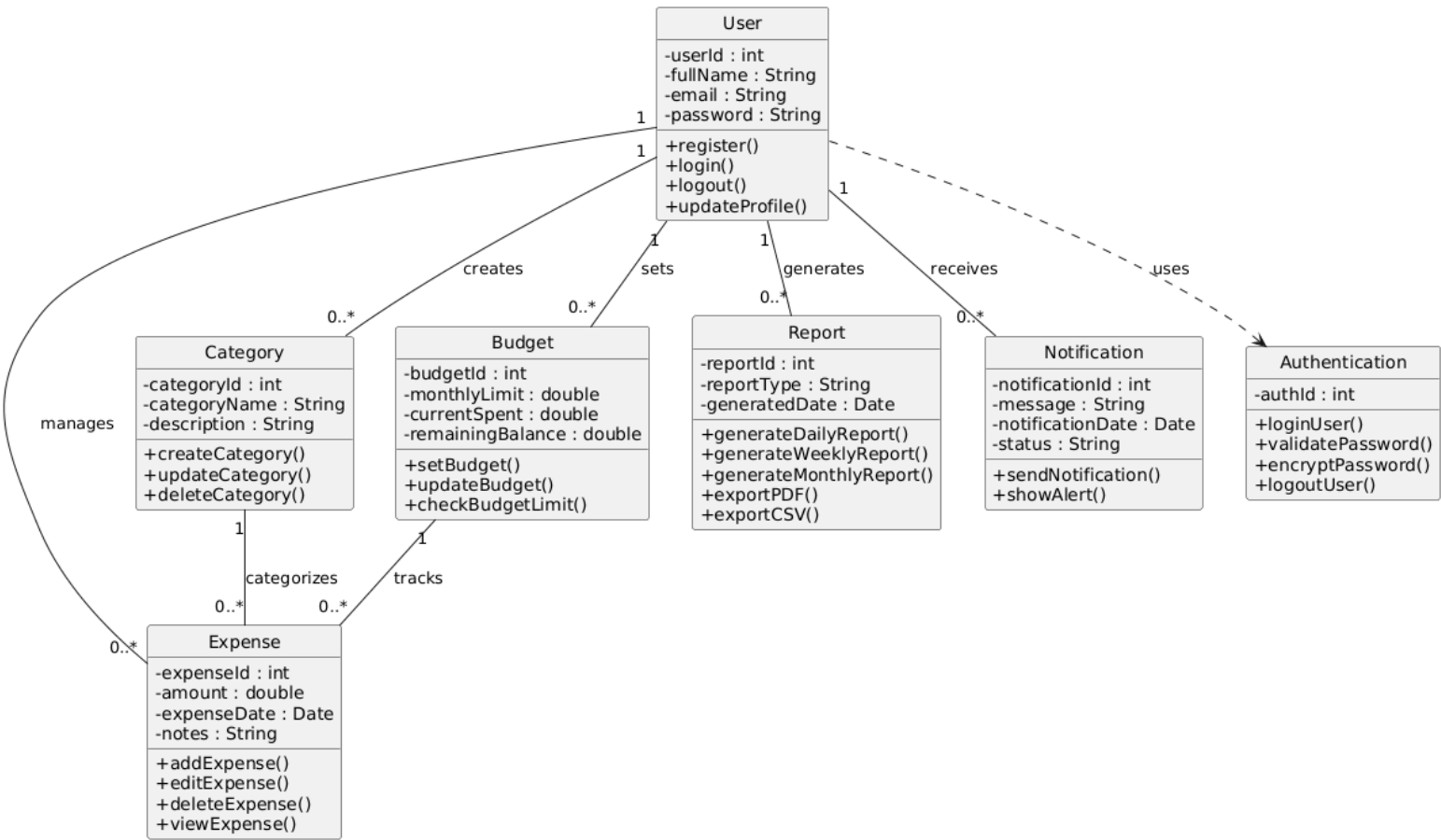
Expense Tracker System - Class Diagram
