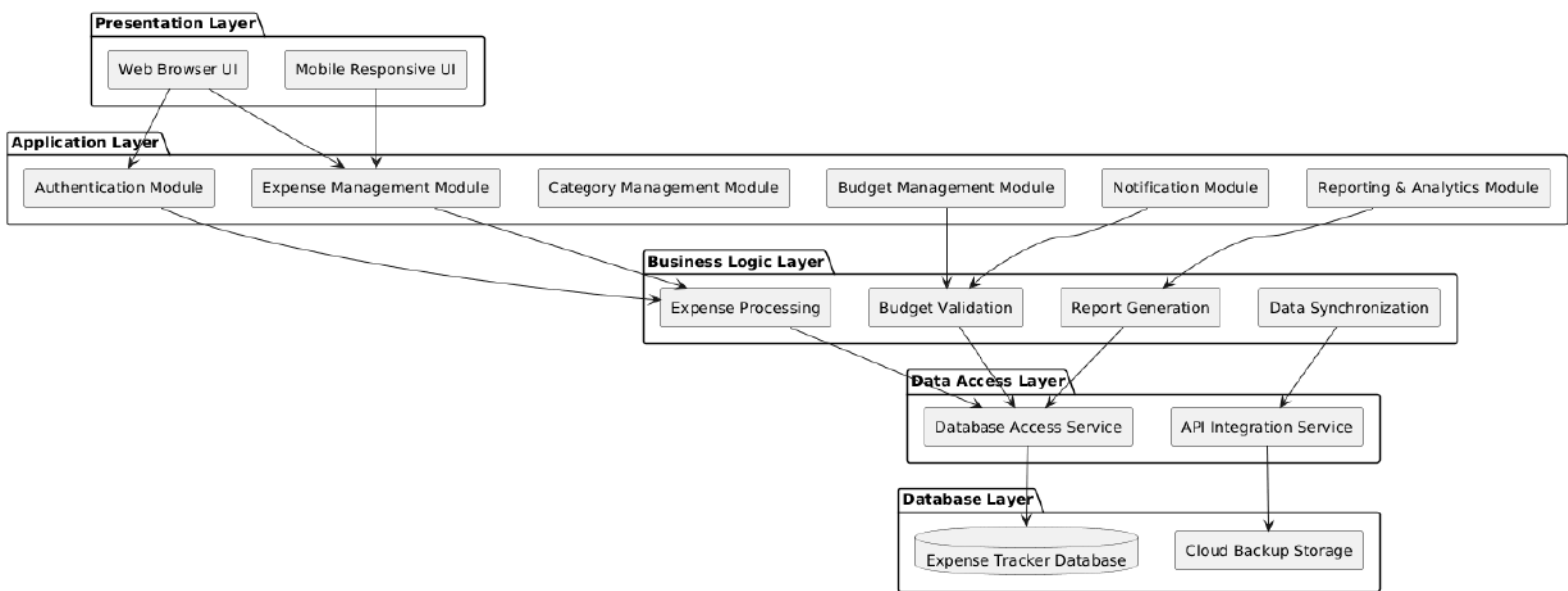
Multilayered Architecture Structure of Expense Tracker System
