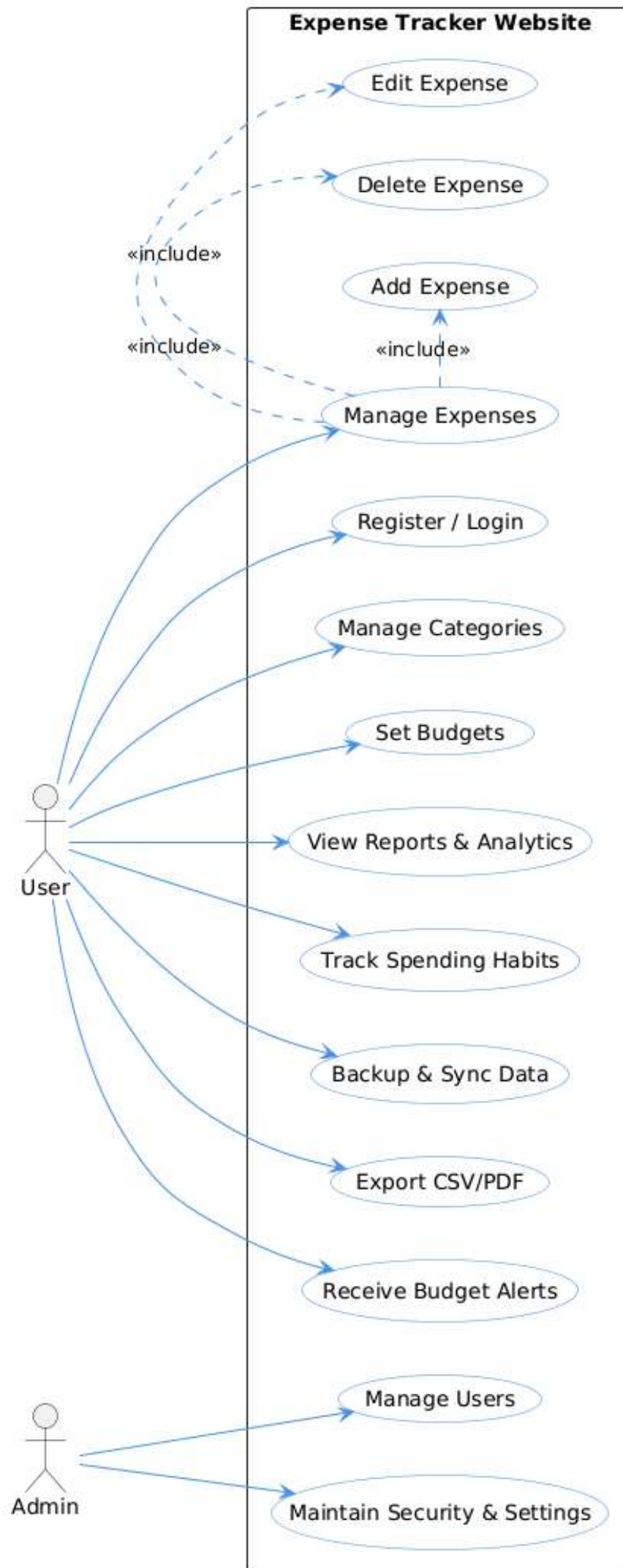
UseCase Diagram For Expense Tracker System
